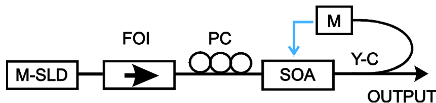
Fig. 2. Schematic sketch of MOPA source.
